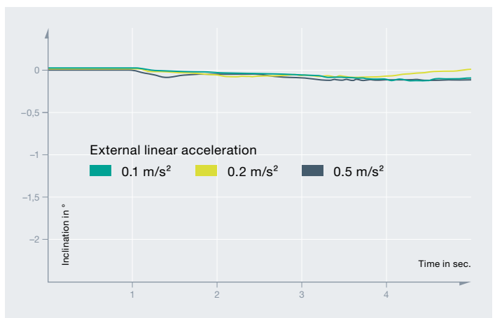
Compensation for external acceleration by F99-Fusion
