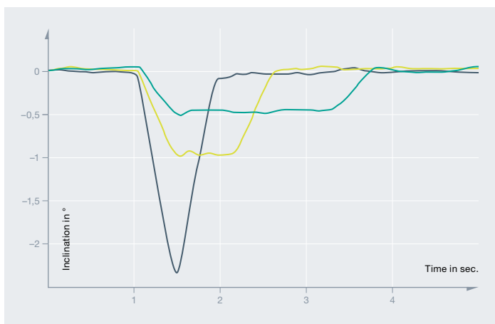
Conventional inclination sensor: measuring error caused by linear acceleration
